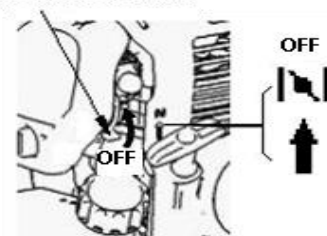
Handle of chock valve
